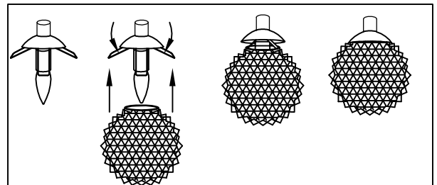
Figure #4--Ball Shade assembly.
