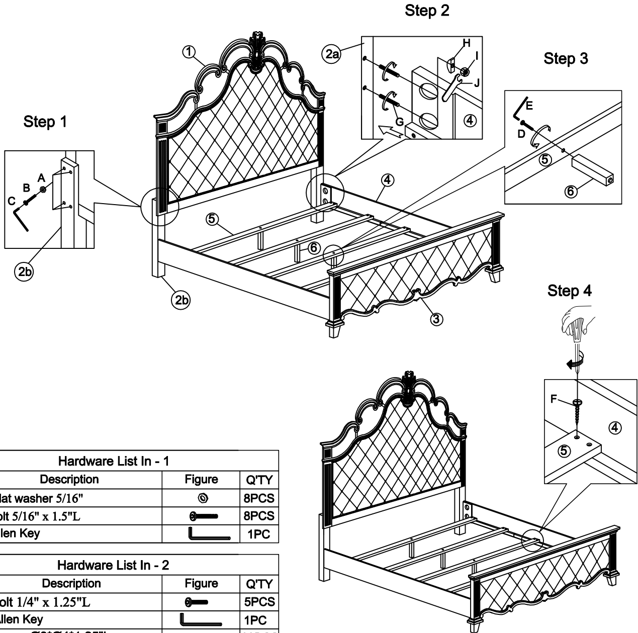
Part List
